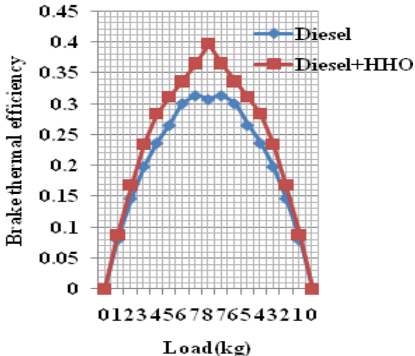
Figure 7. Graph of brake thermal efficiency in percent v/s load in kg.
