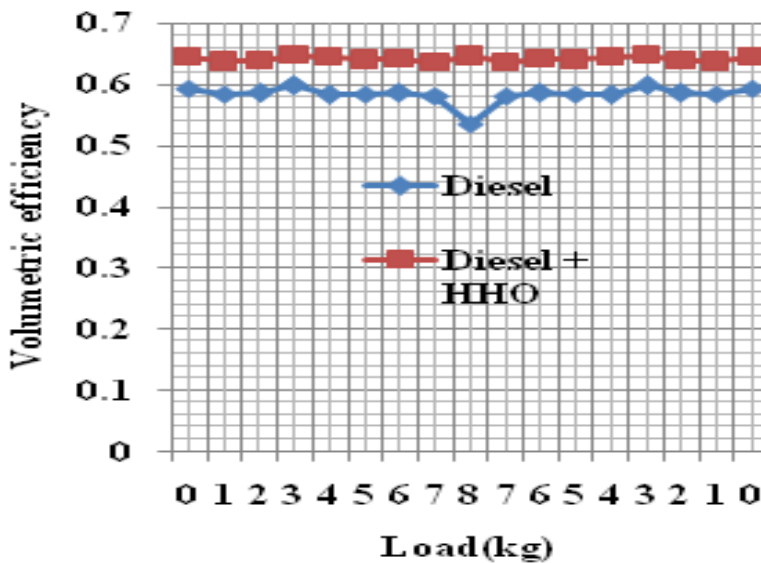
Figure 8. Graph of volumetric efficiency in percent v/s load in kg.
