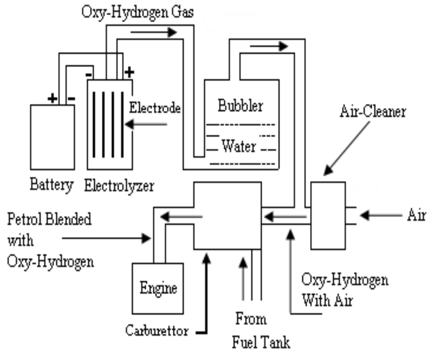
Figure 4. Block diagram of oxy-hydrogen unit mounted on engine.
