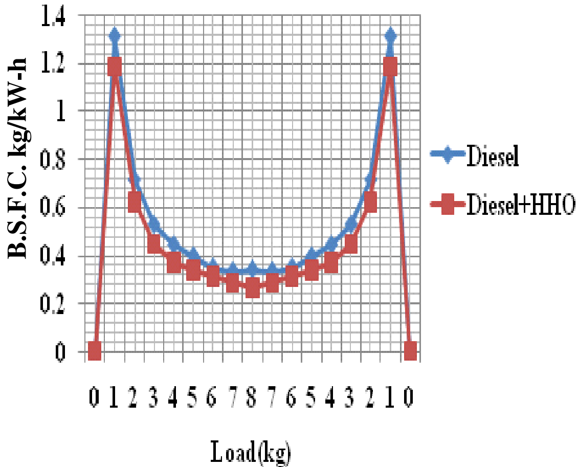
Figure 6. Graph of brake specific fuel consumption in kg/kW-h v/s load in kg.
