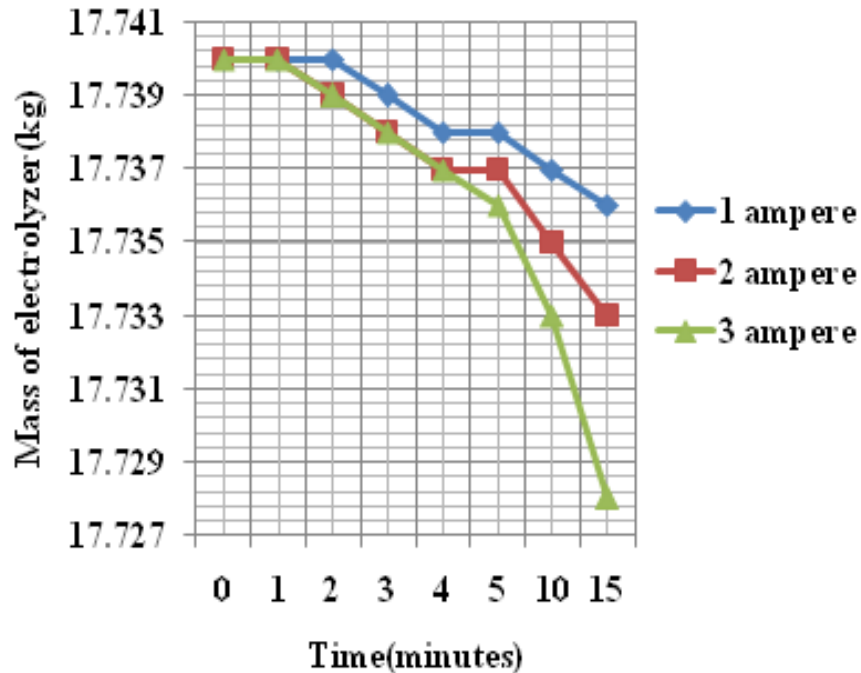
Figure 5. Graph of mass of electrolyser v/s time.
