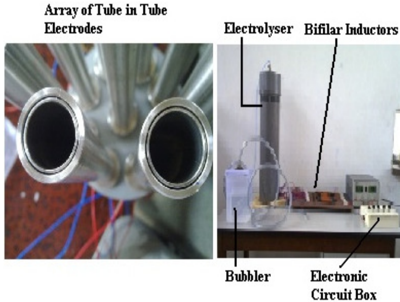
Figure 3. Arrangements of electrodes in second method of electrolyser and other components.
