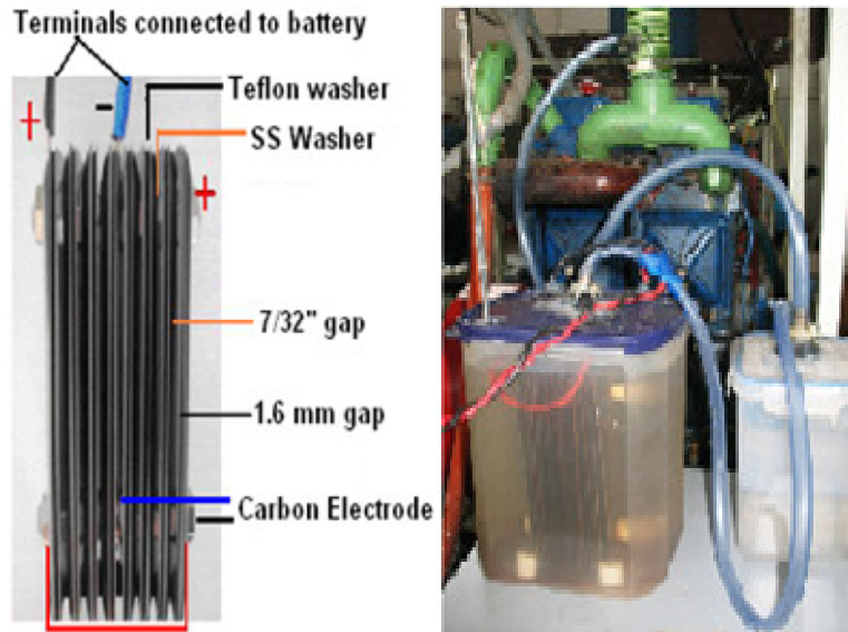
Figure 1. Arrangements of electrodes in first design of electrolyser.
